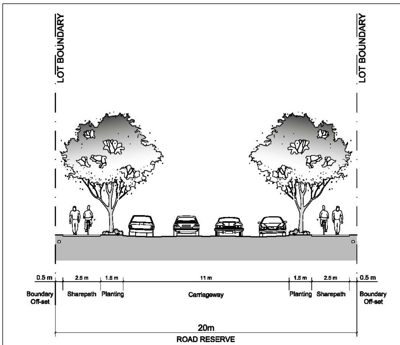
Figure 6-2 Typical industrial street.
