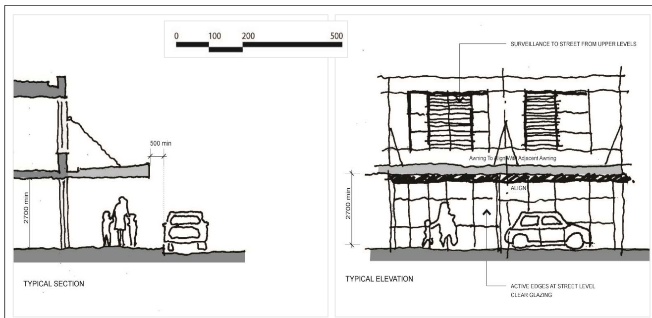
Figure 5-1 Awnings
