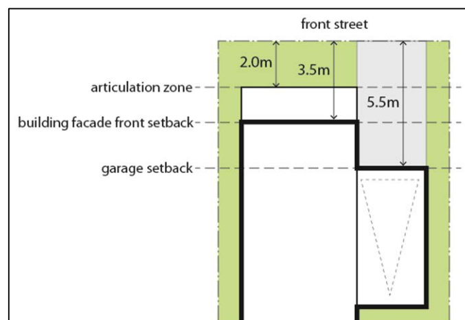
Figure 4-5 Minimum front setbacks for dwellings fronting open space or drainage land.
