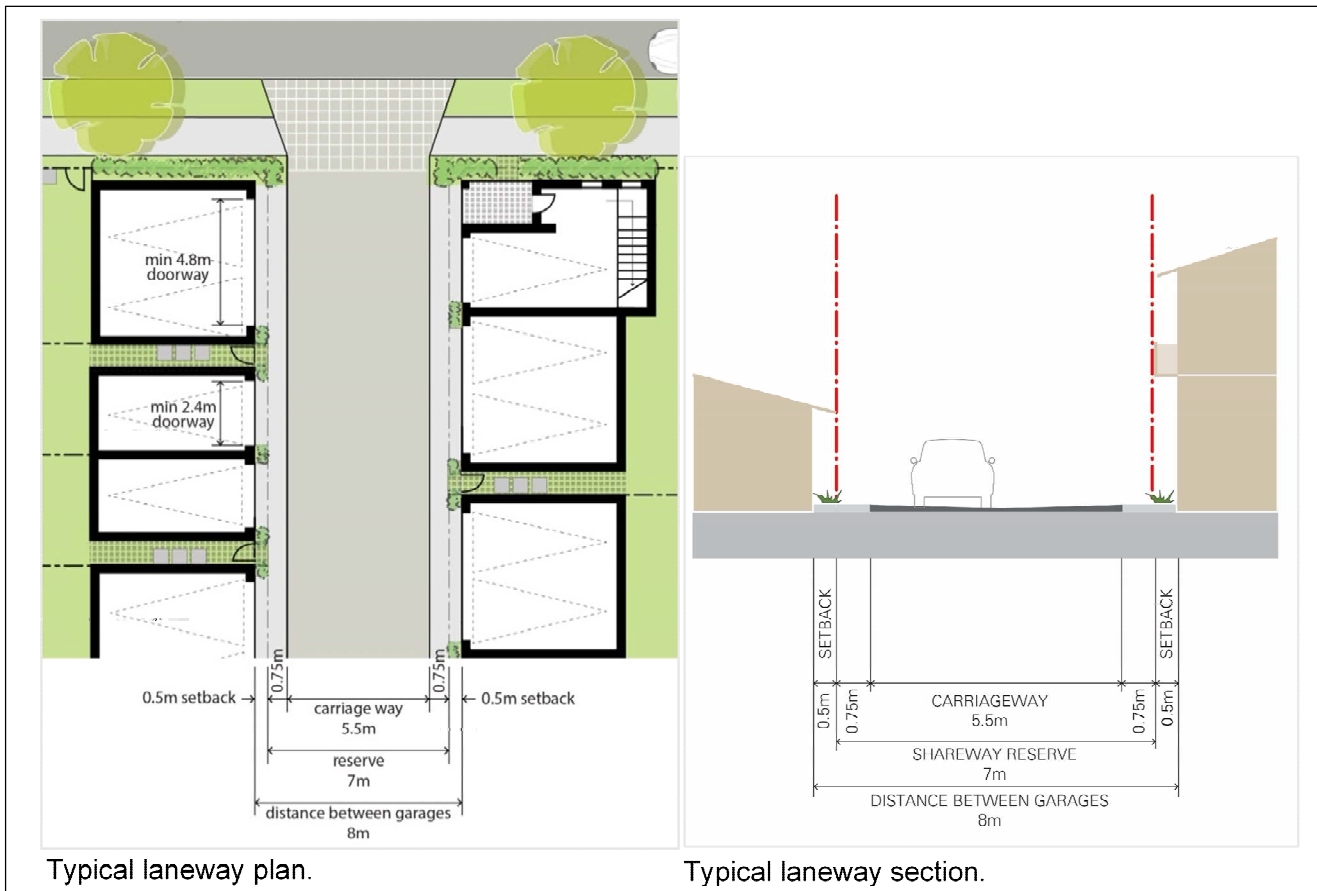
Figure 3-15 Laneway principles.
