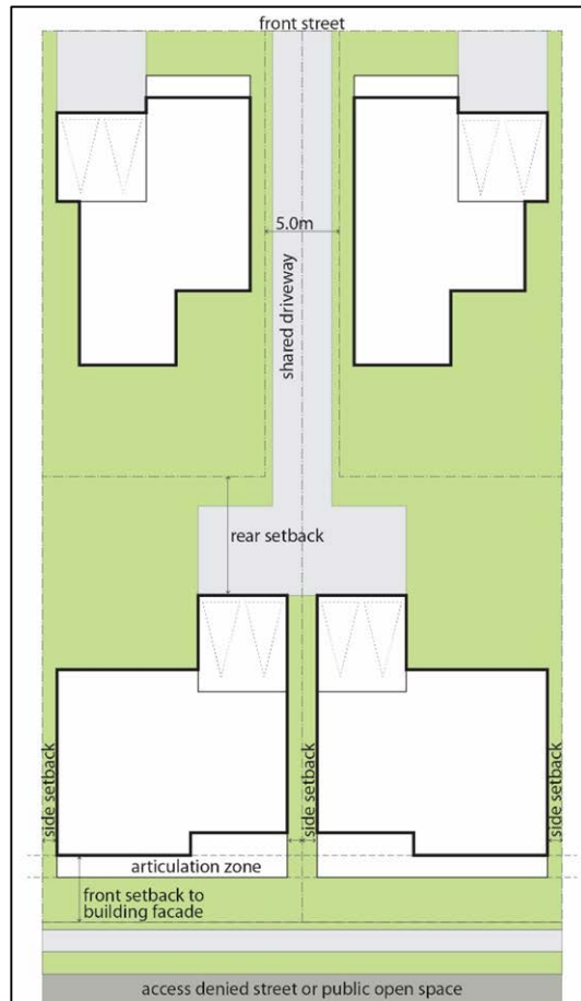
Figure 4-9 Battle axe lot (fronting access denied road) setbacks.
