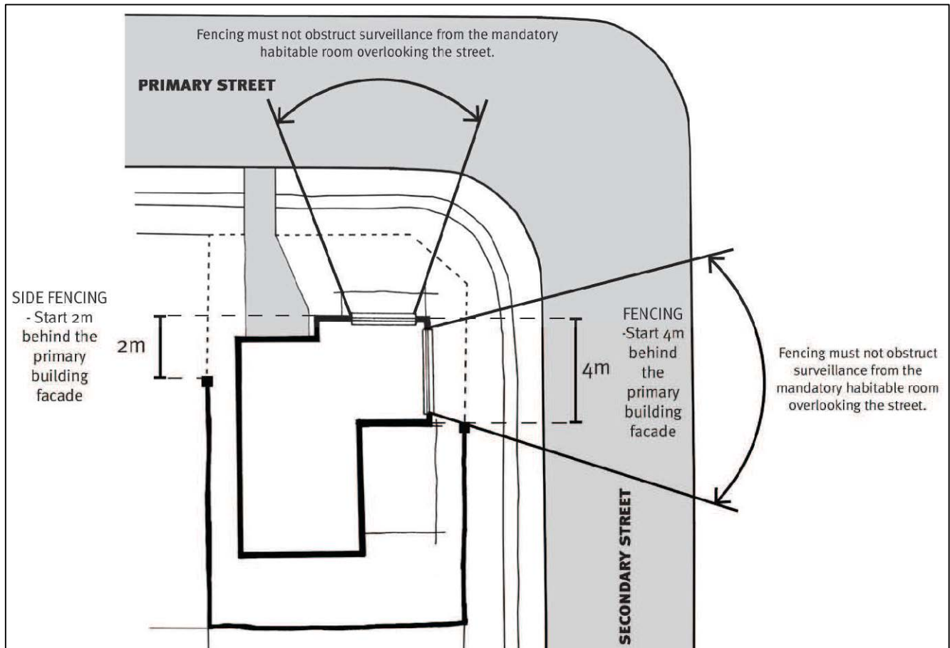
Figure 4-12 Fencing design.
