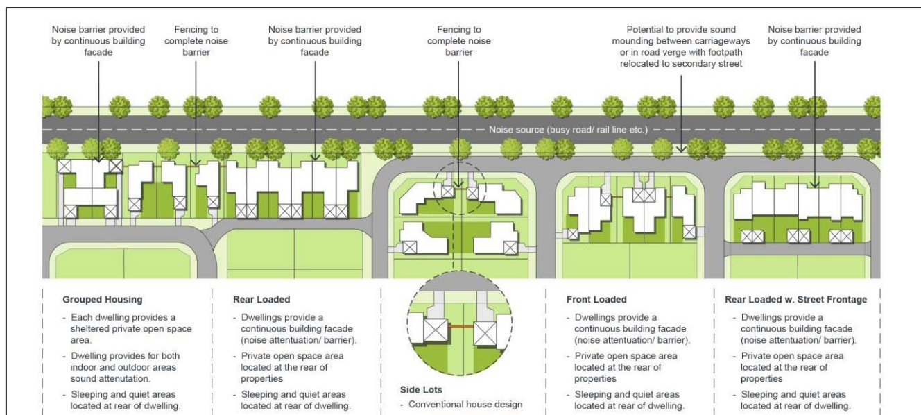
Figure 2-2 Noise from road and rail noise.
