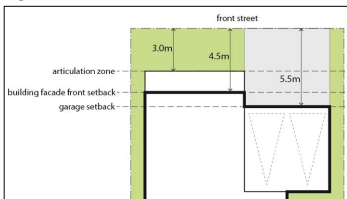
Figure 4-4 Minimum front setback distances.
