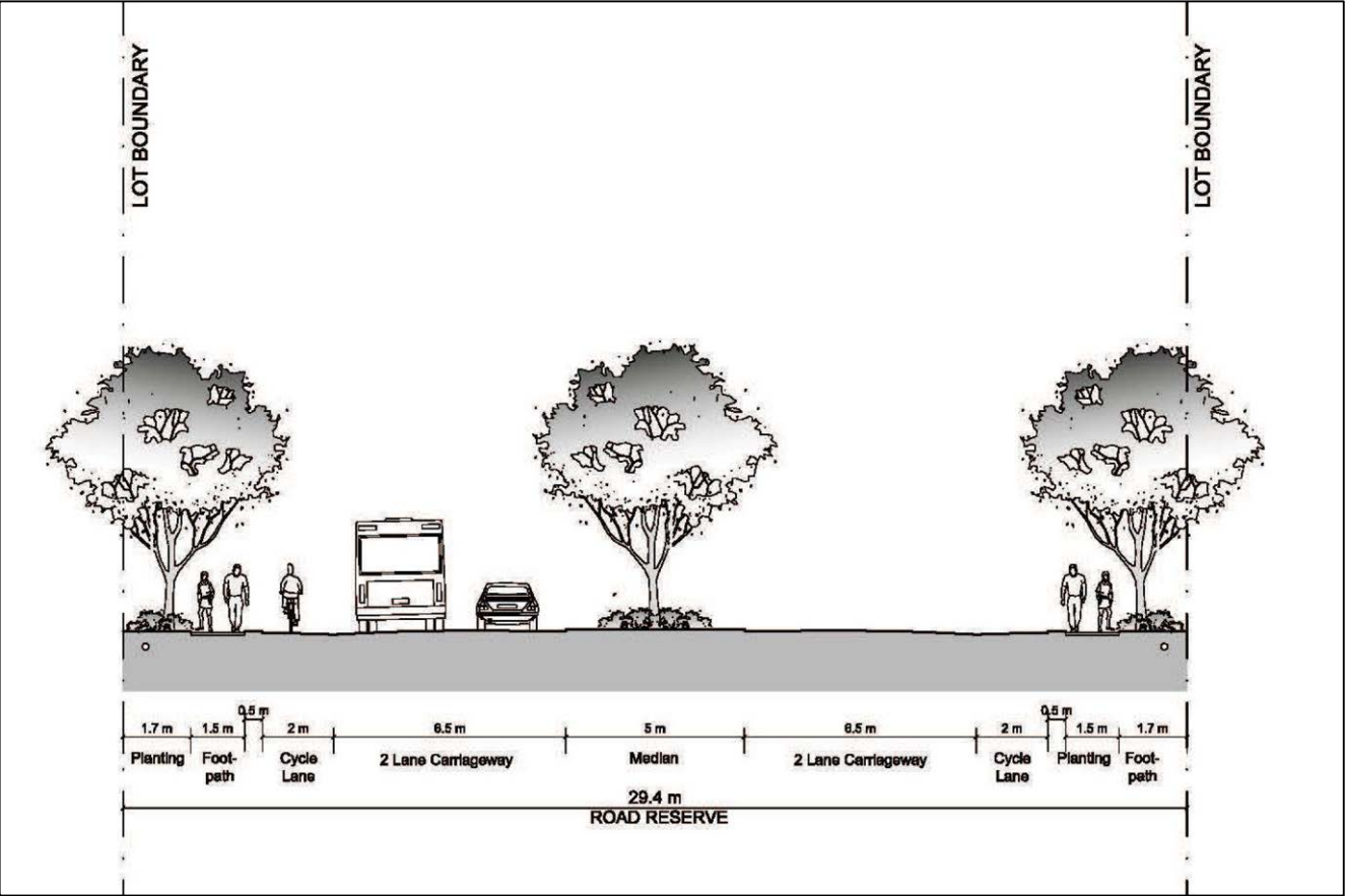
Figure 3-10 Typical transit boulevard.
