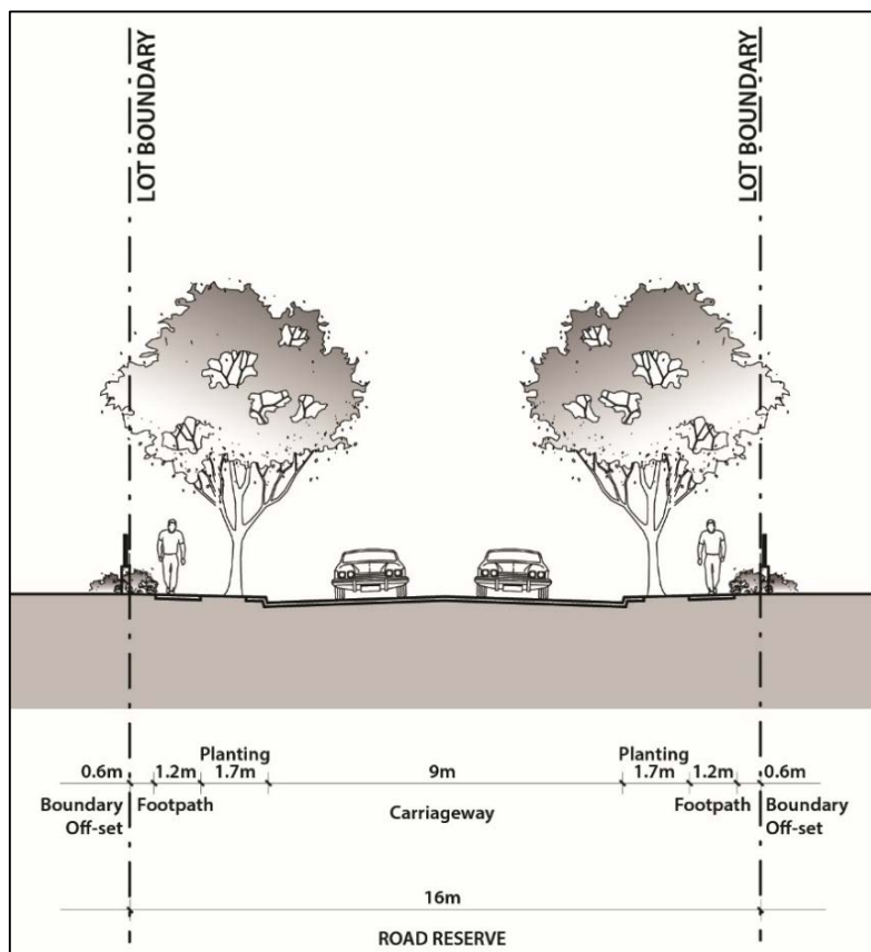
Figure 3-13 Typical primary local street.
