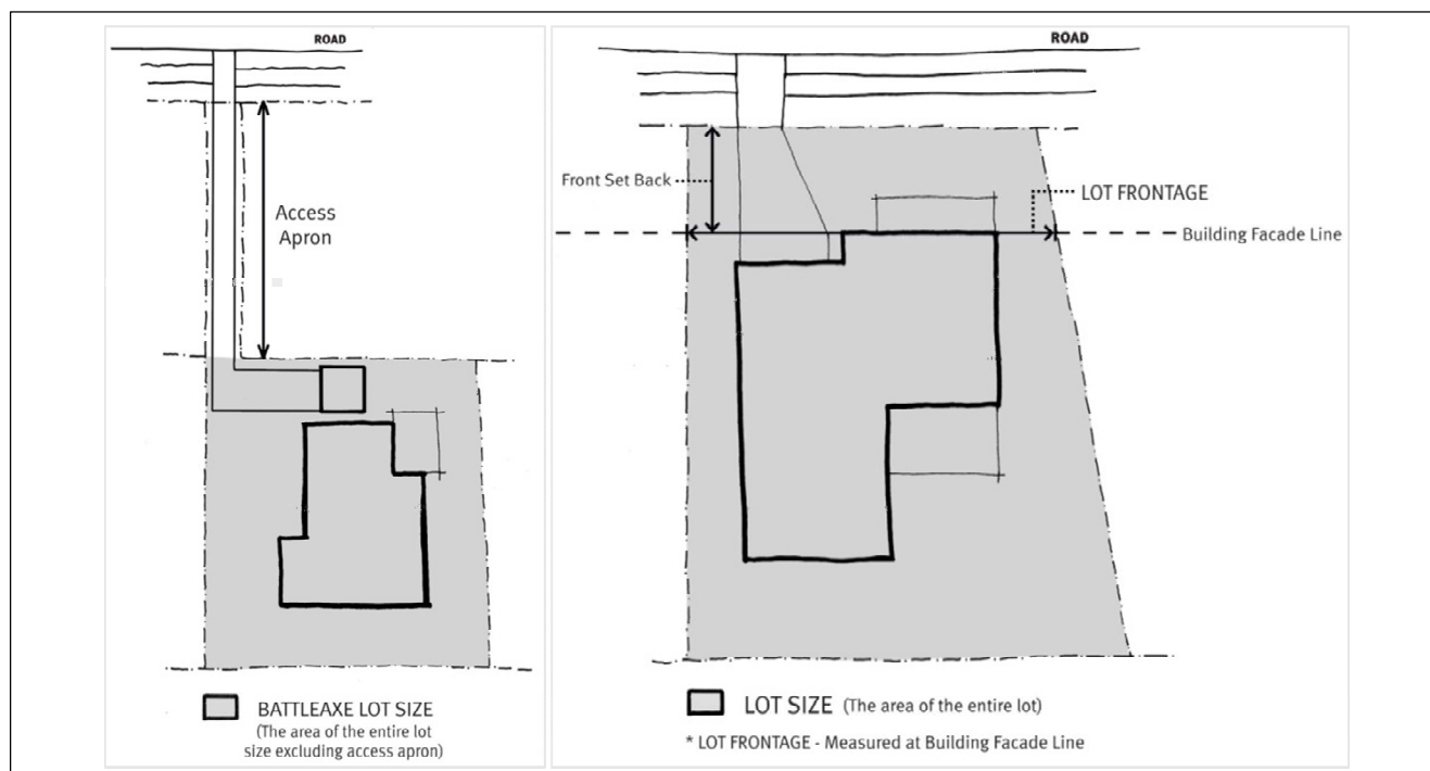
Figure 3-3 Measurement of minimum lot widths and lot area.
