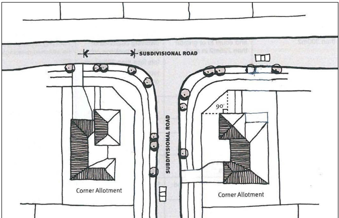
Figure 3-7 Corner Lots
