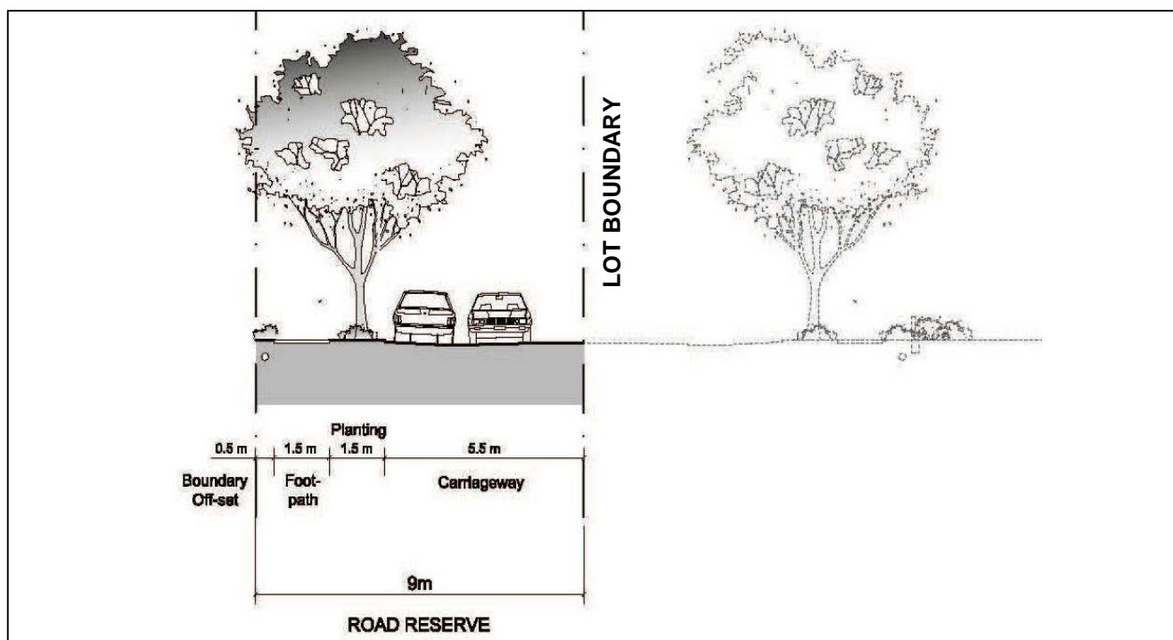
Figure 3-19 Temporary half road width construction.
