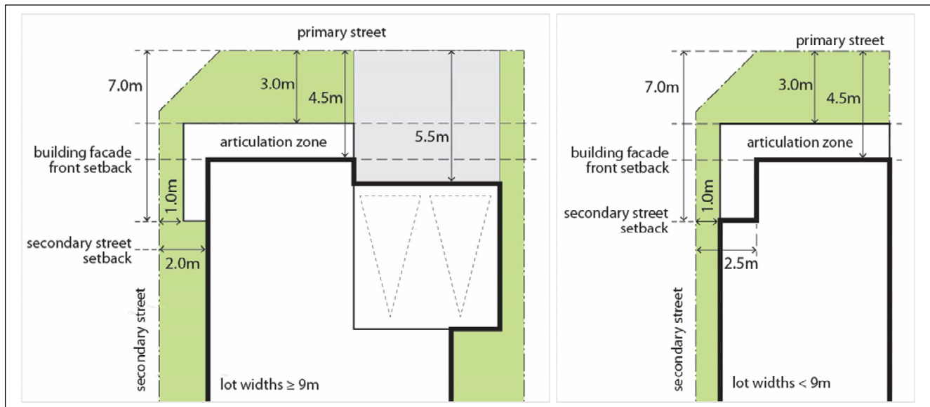
Figure 4-6 Minimum setbacks for corner lot dwellings.
