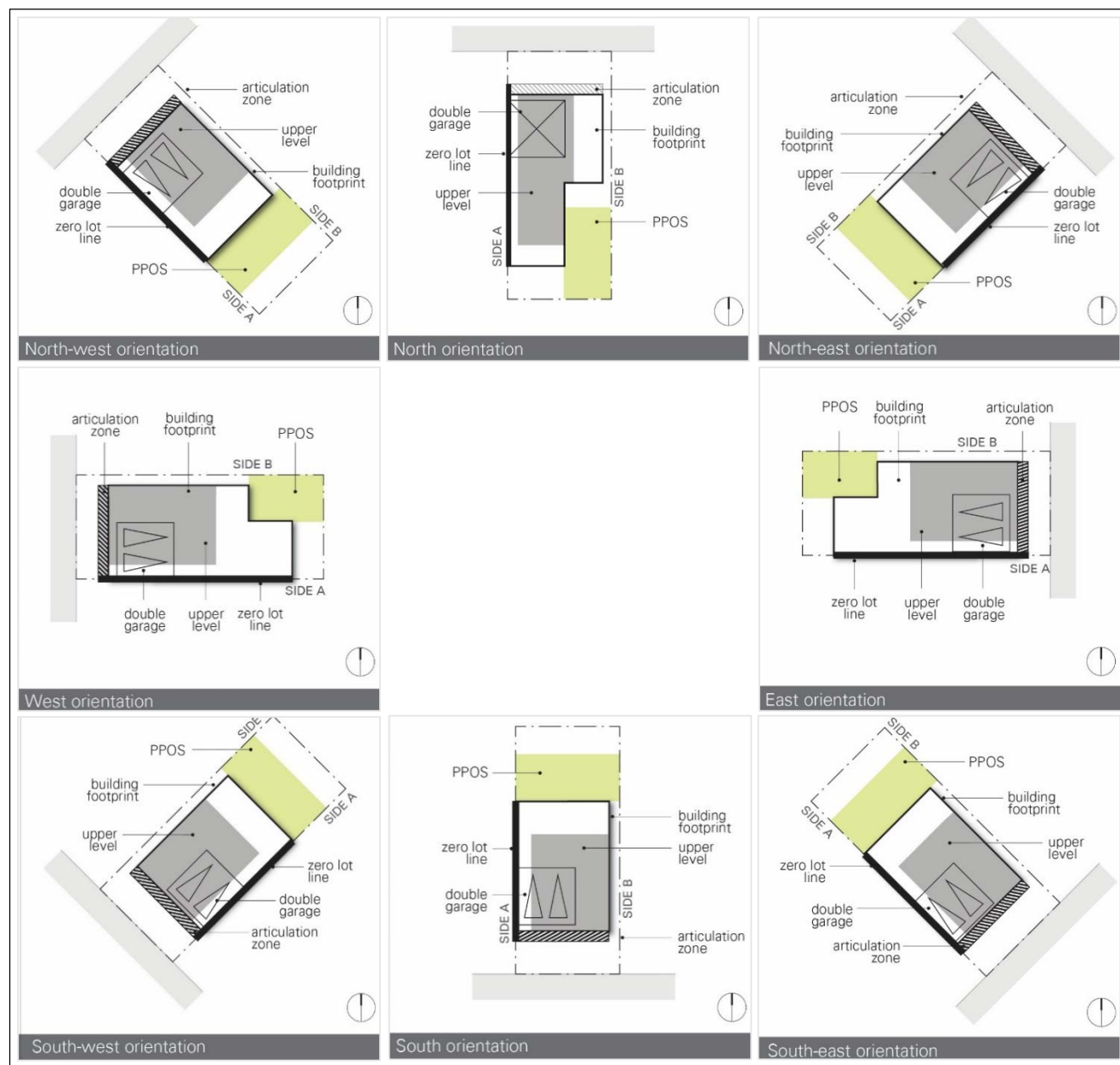
Figure 4-7 Dwelling and open space siting principles for different lot orientations.
