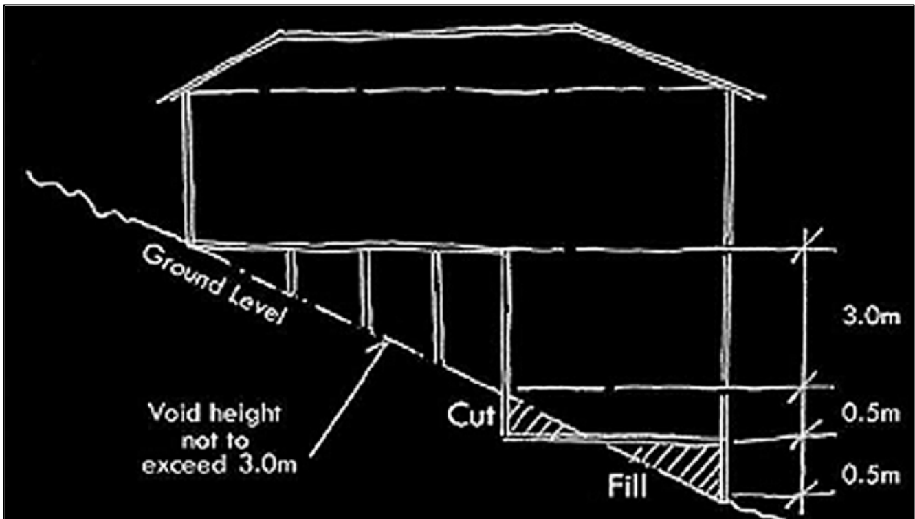
Figure 4-1 Maximum height of voids within residential lots.
