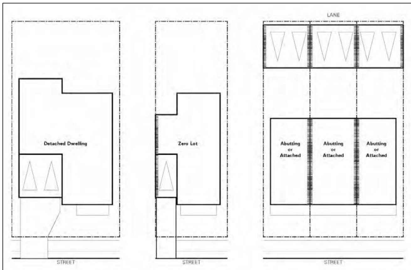
Figure 3 Detached, zero lot line, abutting and attached dwellings.
