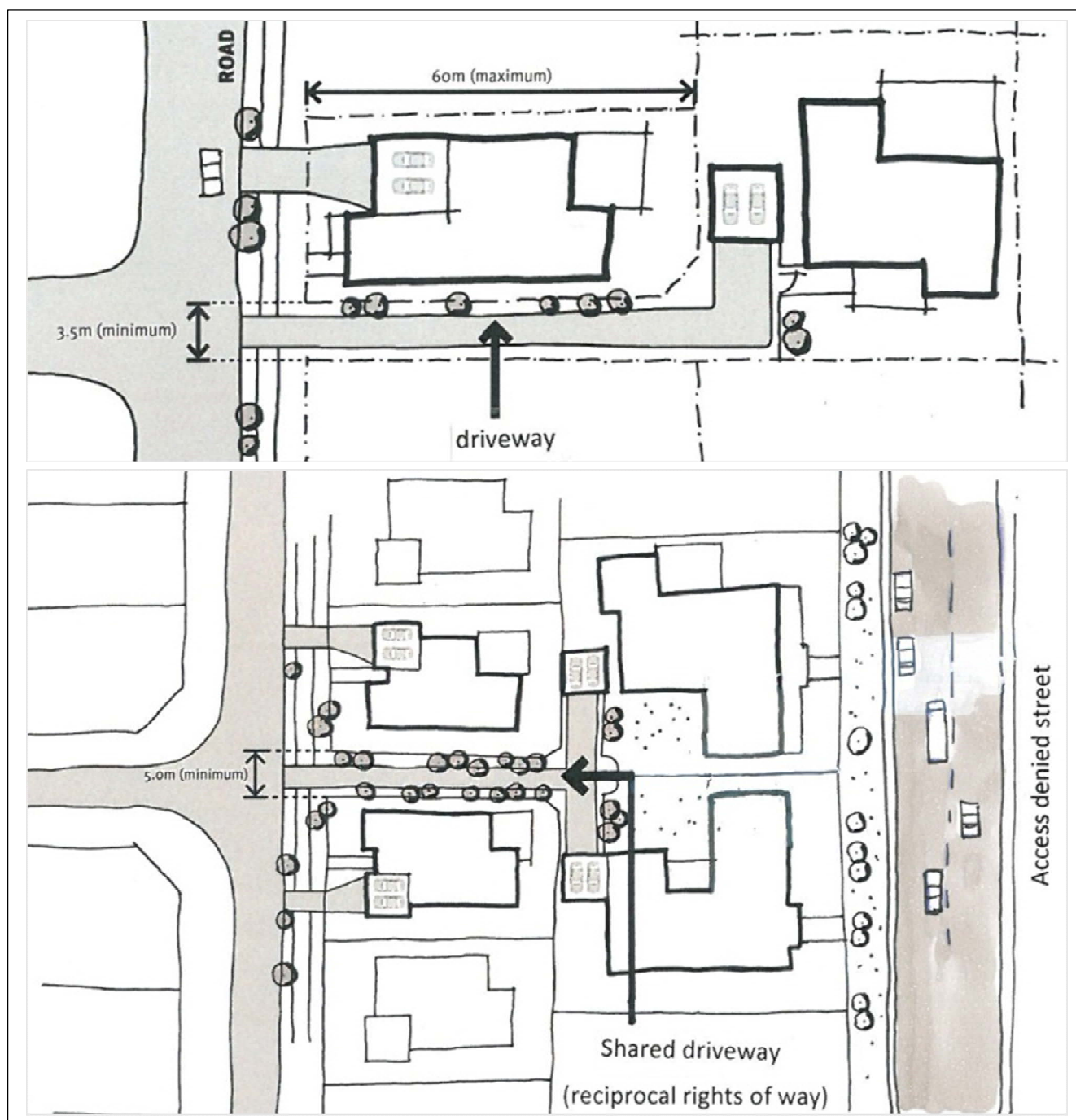
Figure 3-6 Examples of driveways and shared driveways for battle-axe lots.
