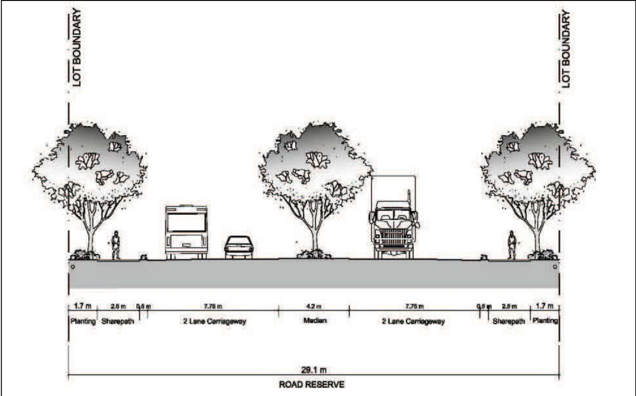
Figure 3-11 Typical sub-arterial road.
