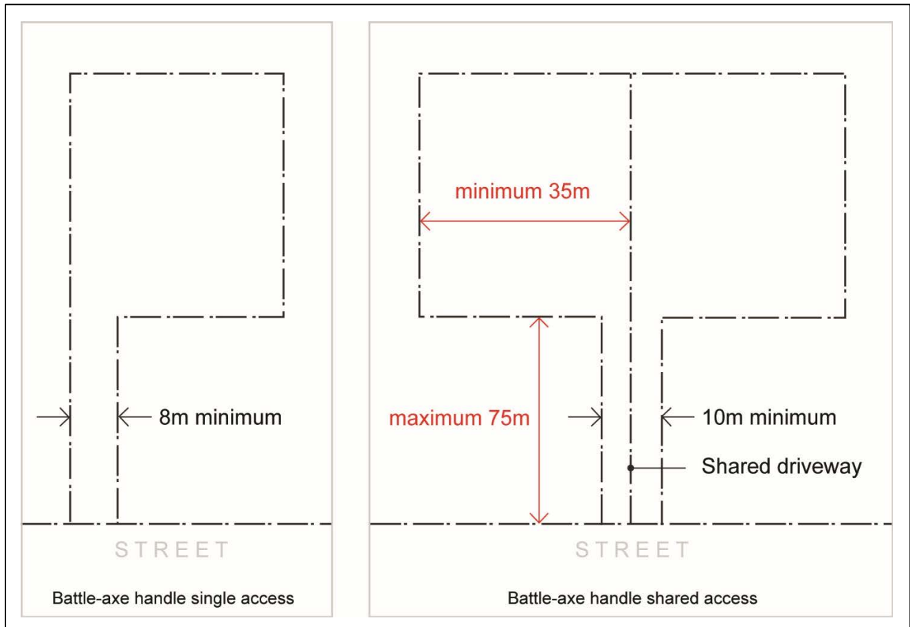
Figure 6-1 Battle axe lot dimensions.
