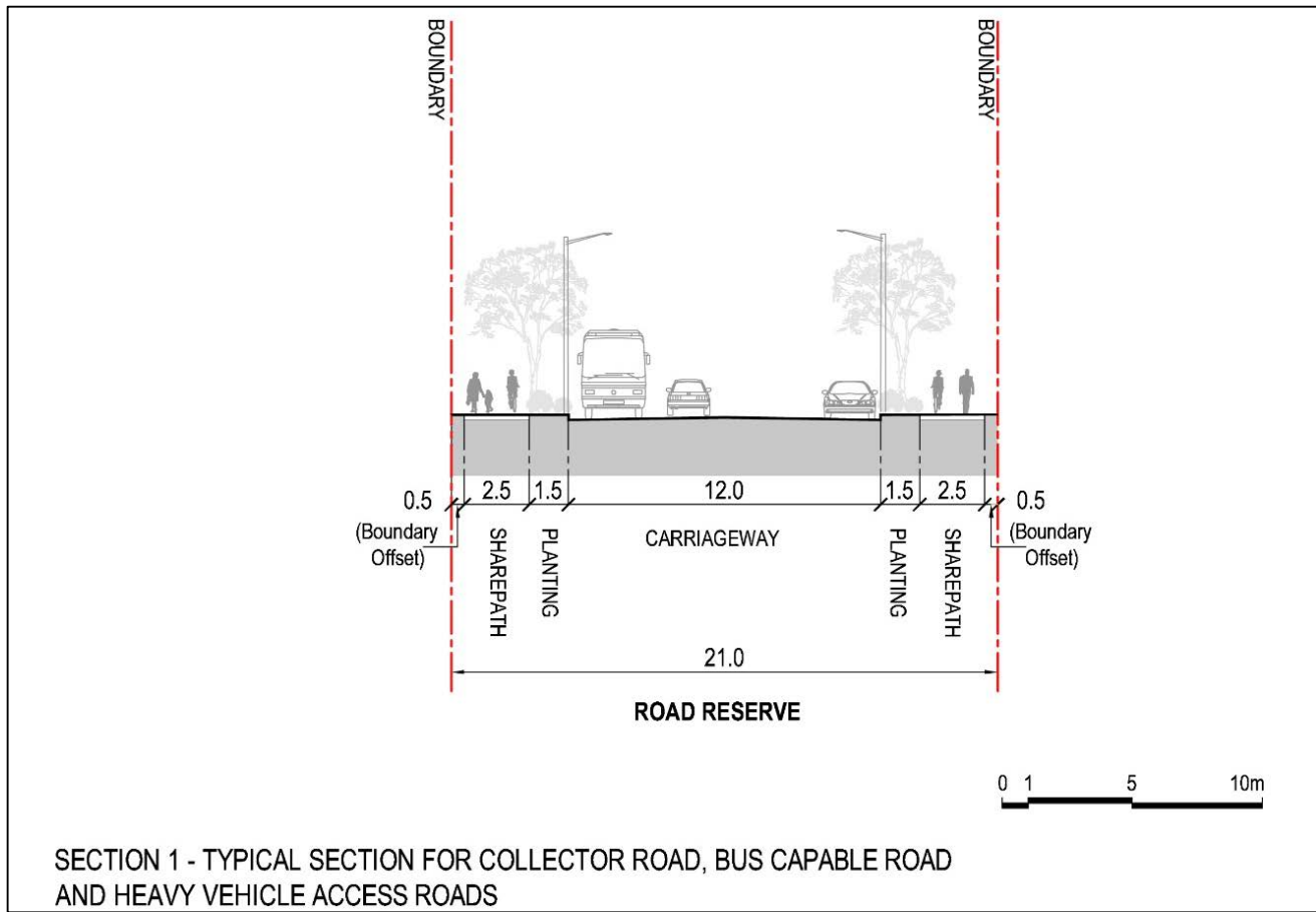
Figure 3-12 Typical collector road.
