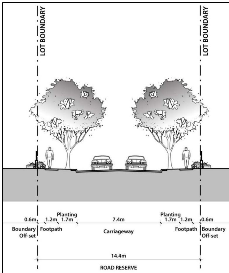
Figure 3-14 Typical local street.
